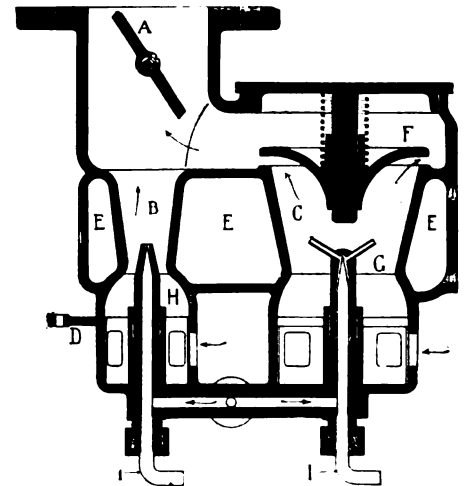
Details of the Willet Carbureter.
